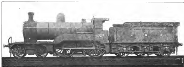
Fig. 5043. Eight-Wheel, Four-Coupled Locomotive. Great Northern Railway. Cylinders 17½ in. x 26 in.; Working Steam Pressure 170 lbs. per sq. in.; Total Heating Surface 1,219.8 sq. ft.; Diameter of Drivers 80 in.; Weight on Drivers 69,440 lbs.; Total Weight 106,400 lbs.
